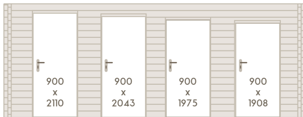
Doors dimensions
